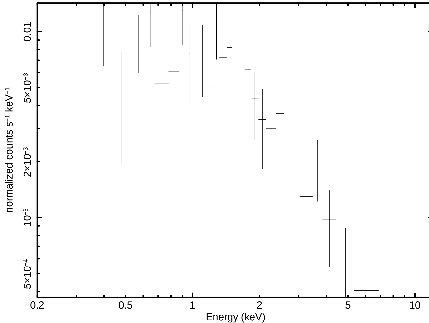
Source 12 minus background (P0124711401M2S003SRSPEC000C)
