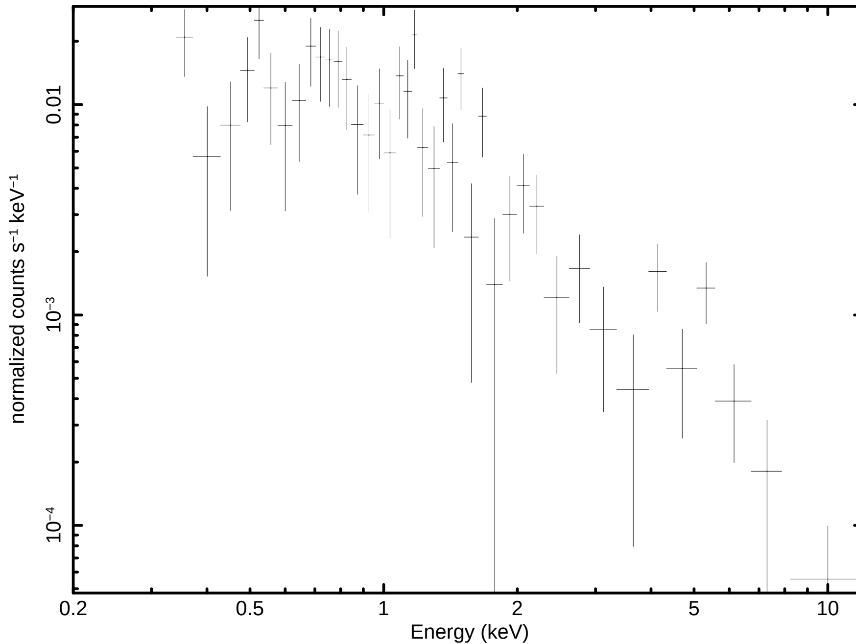
Source 12 minus background (P0124710501PNS001SRSPEC000C)
