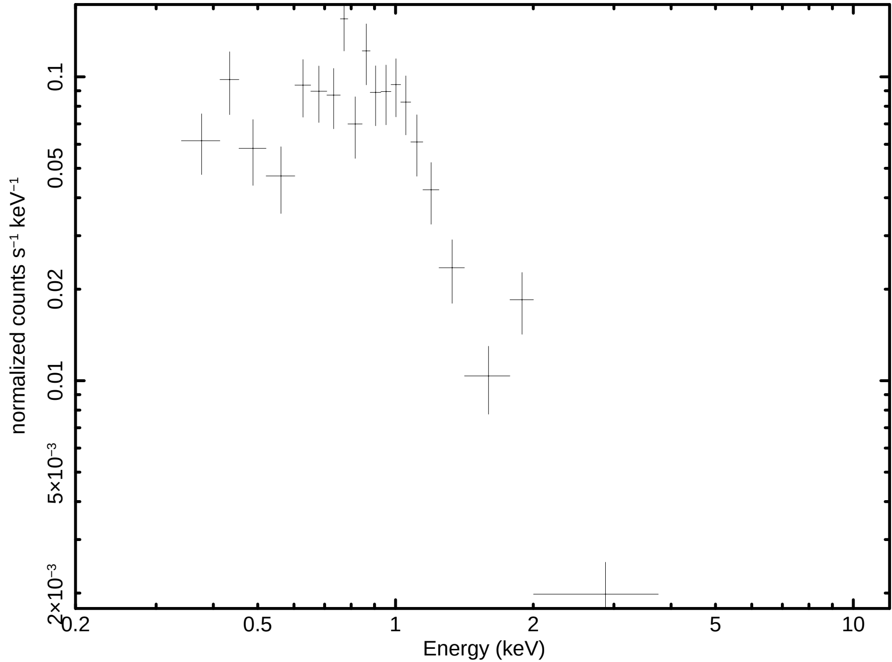
Source 1 minus background (P0002740101PNS003SRSPEC0001)
